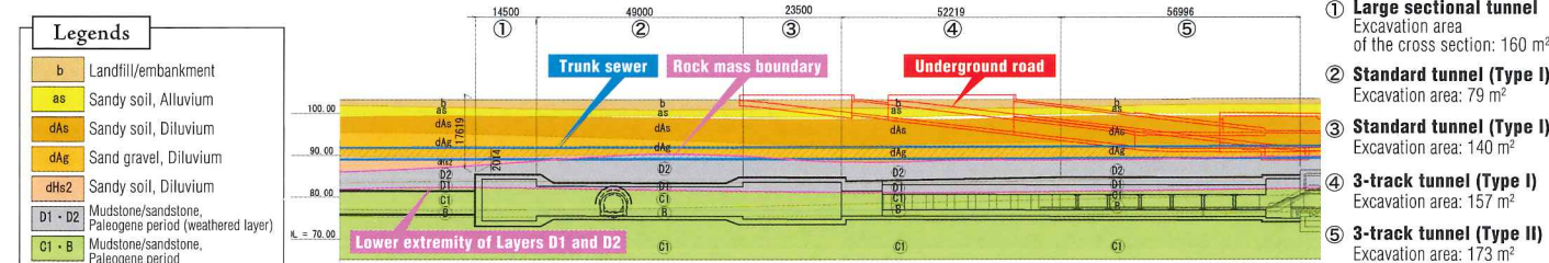
Fig. 2 Geological profile of the NATM tunneling section
