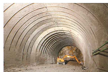
Photo 2 Smoothing of shotcrete surface (up front: WT section, in the back: non-WT section)
