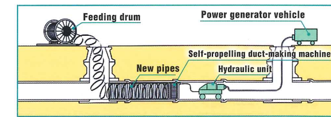
Fig. 2 How to construct sewer pipes
