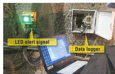
Photo 2 Data logger and LED alert signal
