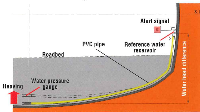
Fig. 1 Schematic drawing of invert displacement measurement
