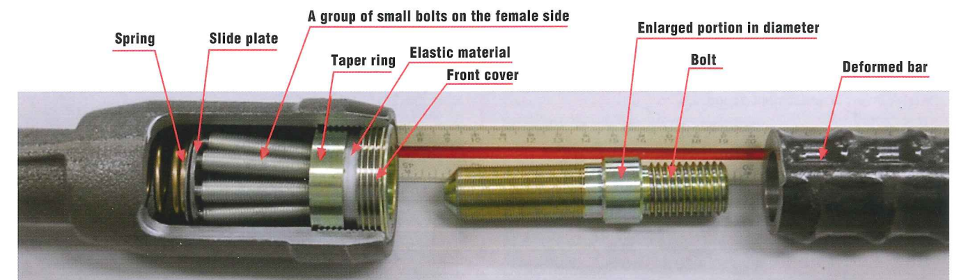
Fig. 2 Structure of the SB joint
