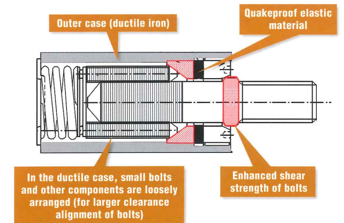
Fig. 1 Schematic diagram of the SB joint
