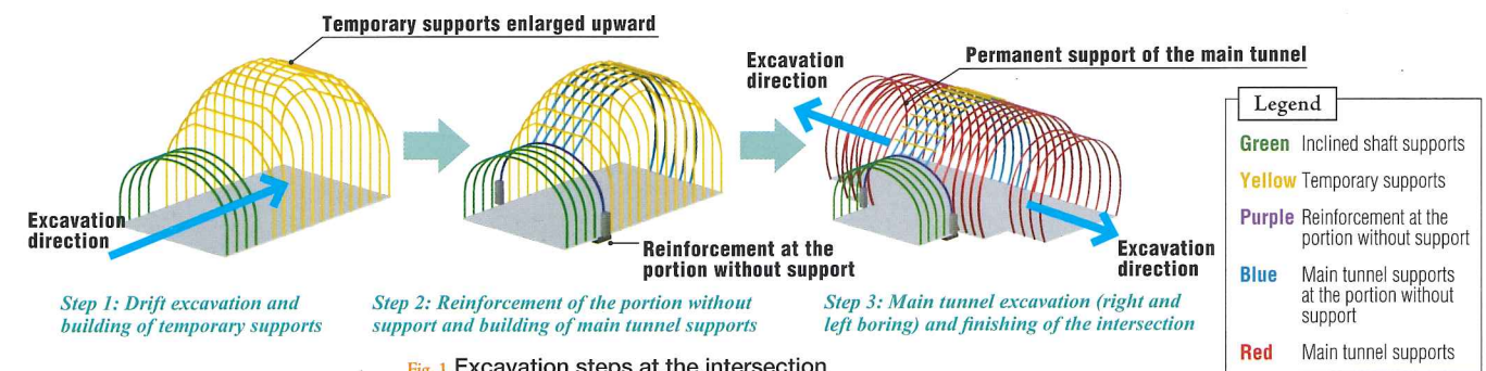
Fig. 1 Excavation steps at the intersection
