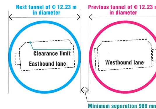
Fig. 2 Cross-section
