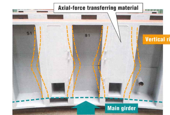
Fig. 3 Structure of the segment (compression-deformation model)
