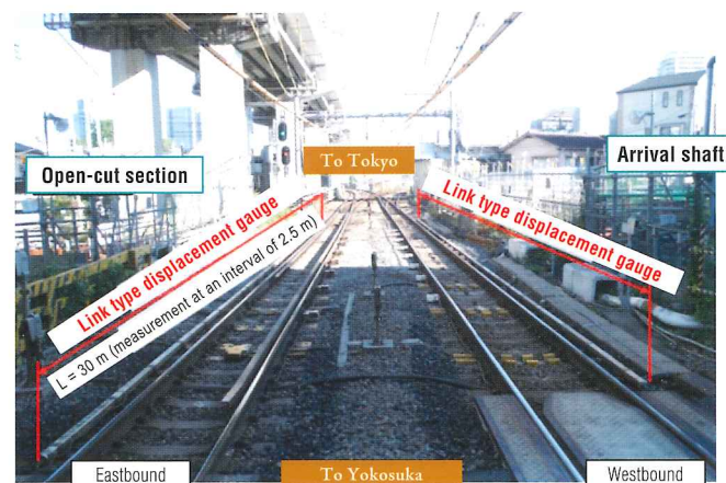
Photo 3 Track displacement measurement at the railway track crossing point
