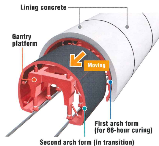
Fig. 1 Schematic diagram of the special formwork
