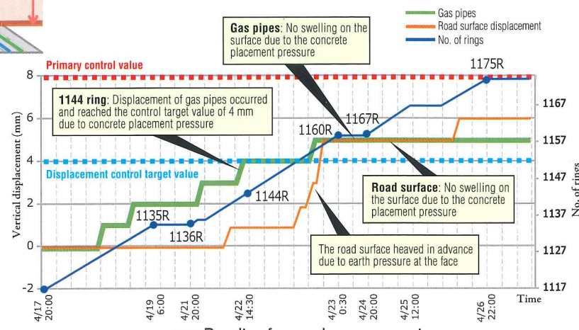
Fig. 2 Results of manual measurements of displacement for the road surface and gas pipes
