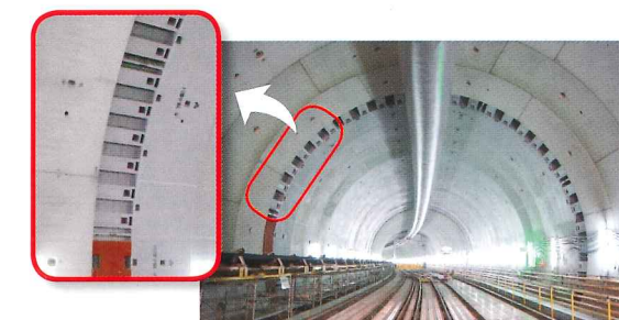
Fig. 4 View of the construction
