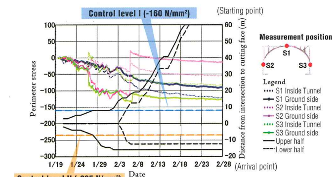
Fig. 2 Changes generating stress at the time of reinforcing the missing part
