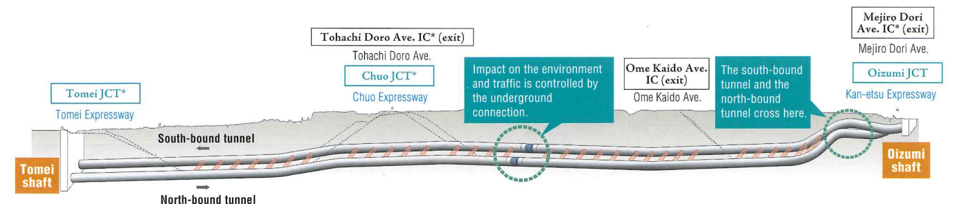
Fig.2 Main shield tunnel
