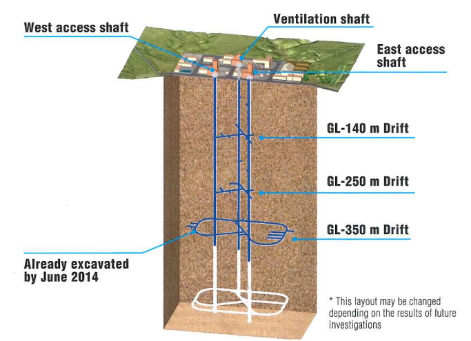
Fig. 1 Layout of the Horonobe Underground Research Laboratory
