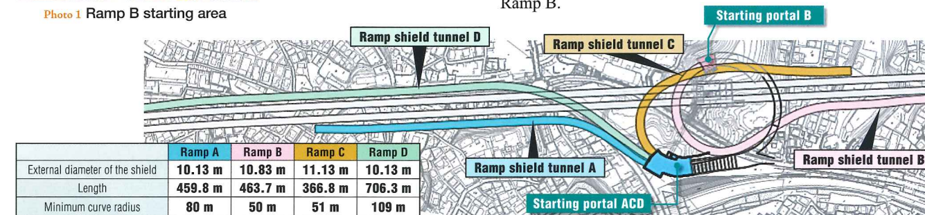
Fig. 1 Overall ground plan of the Baba Interchange
