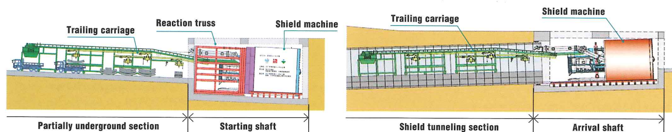
Fig. 1 Diagram of shield boring starting and ending on the ground surface
